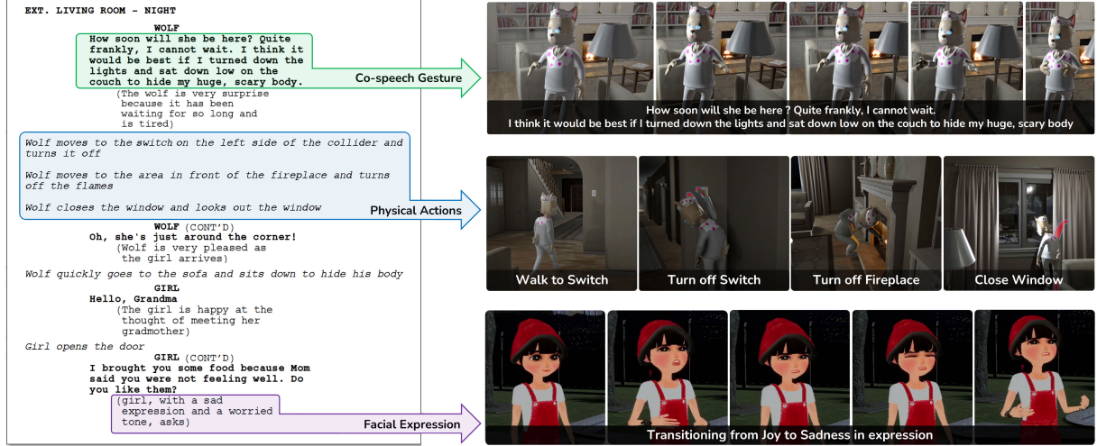
Fig. 11 Illustrative scenario “Little Red Riding Hood”, the ASAP system produces a cartoon-like pre-visualization based on the screenplay. This pre-visualization encompasses key moments such as the wolf demonstrating co-speech gestures while delivering his monologue, the wolf taking a series of physical actions to interact with virtual props, and the girl displaying a range of changing facial expressions.
