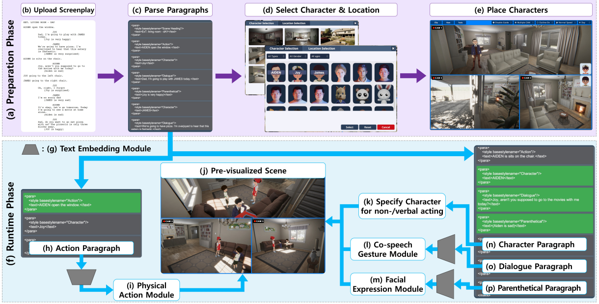
Fig. 3 The overall process of the ASAP system is to understand/interpret the screenplay and subsequently generate (or animate) the behavior of virtual characters in the 3D pre-visualization. The first line (purple box) illustrates the (a) Preparation phase of the ASAP system, which consists of the following steps: (b) The written screenplay is uploaded to the ASAP system; (c) The ASAP parses the screenplay into different paragraphs, including Action , Character , Dialogue , and Parenthetical ; (d) Selecting a location and characters to demonstrate a screenplay; and (e) Placing characters in the selected location. In the second line (blue box), the (f) Runtime phase of the ASAP system is displayed, and (j) previz is sequentially generated by the screenplay. The paragraph of the screenplay is sequentially passed to each pertinent module: (h) Action paragraph passed to the (i) physical action module; (n) Character paragraph is used to (k) specify the target for applying the animation generated from the following paragraph; (o) Dialogue paragraph passed to the (l) co-speech gesture module; (p) Parenthetical paragraph pass to the (m) facial expression module; and lastly, (g) the grey trapezoid indicates the module for text embedding.
