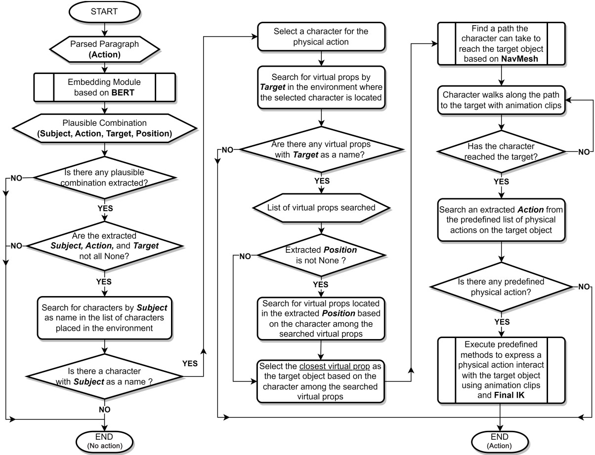
Fig. 8 The flowchart illustrates the process of generating procedural animation (i.e., physical action) by using the plausible action combinations extracted from action paragraphs in the screenplay. The left-side endpoint indicates that the action paragraph lacks sources to generate physical actions, whereas the right-side endpoint indicates the successful generation of physical actions for virtual characters.
