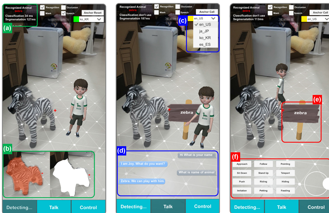
Figure 7. Overview of our multimodal mobile AR system. (a) Recognizing real objects; (b) displaying the segmentation mask and placing the silhouette mesh; (c) supporting multi-language; (d) Voice chat between a user and a virtual human based on knowledge database [3]; (e) Placement of persistent anchor based on spatial mapping [3]; and (f) realistic interactions with real animal dolls using the silhouette mesh.
