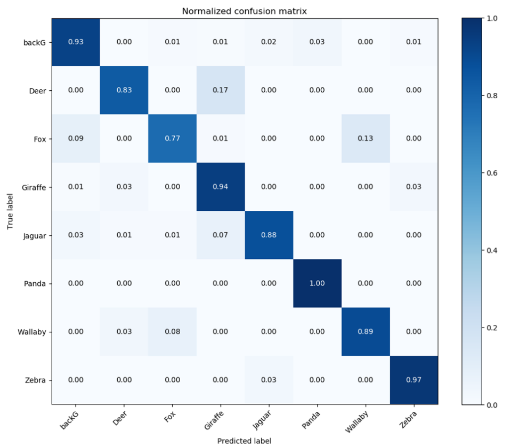
Figure 3. Recognition accuracy with seven animal dolls.
