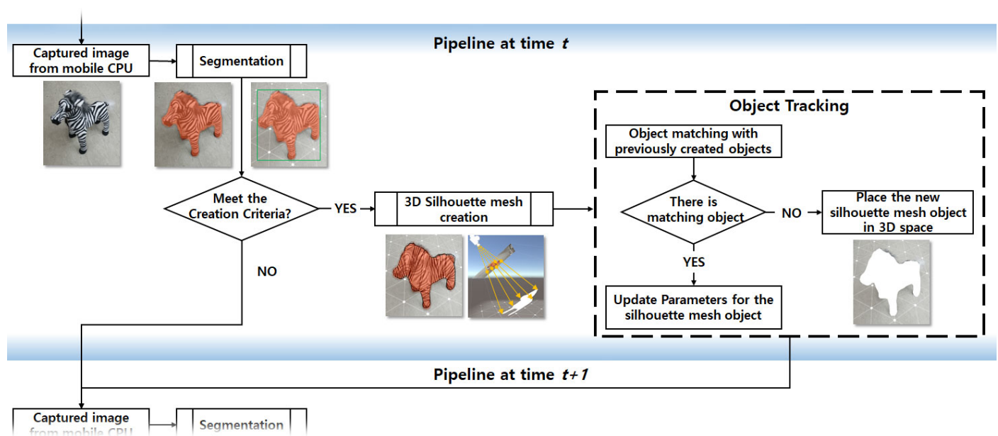
Figure 5. Overview of our system's main pipeline and detailed silhouette mesh update process.
