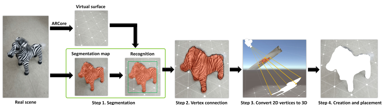
Figure 4. Overview of our silhouette mesh creation process. First, we detect the floor from the phone camera and place the virtual surface on it. At the same time, images from the camera are fed into our network to segment and recognize the interactable object. Based on the segmented region, bounding boxes are generated. For each object, we create vertices along the boundary of the segmented area on the image plane. Then we cast a ray from the camera toward the midpoint of the bottom line of the bounding box and we calculate the distance between the camera and the collision position on the virtual surface. Similarly, we cast rays toward all vertices on the image plane and set the 3D vertices that have equal distance with regard to the camera. Finally, the silhouette mesh is formed (see Section 3.2).
